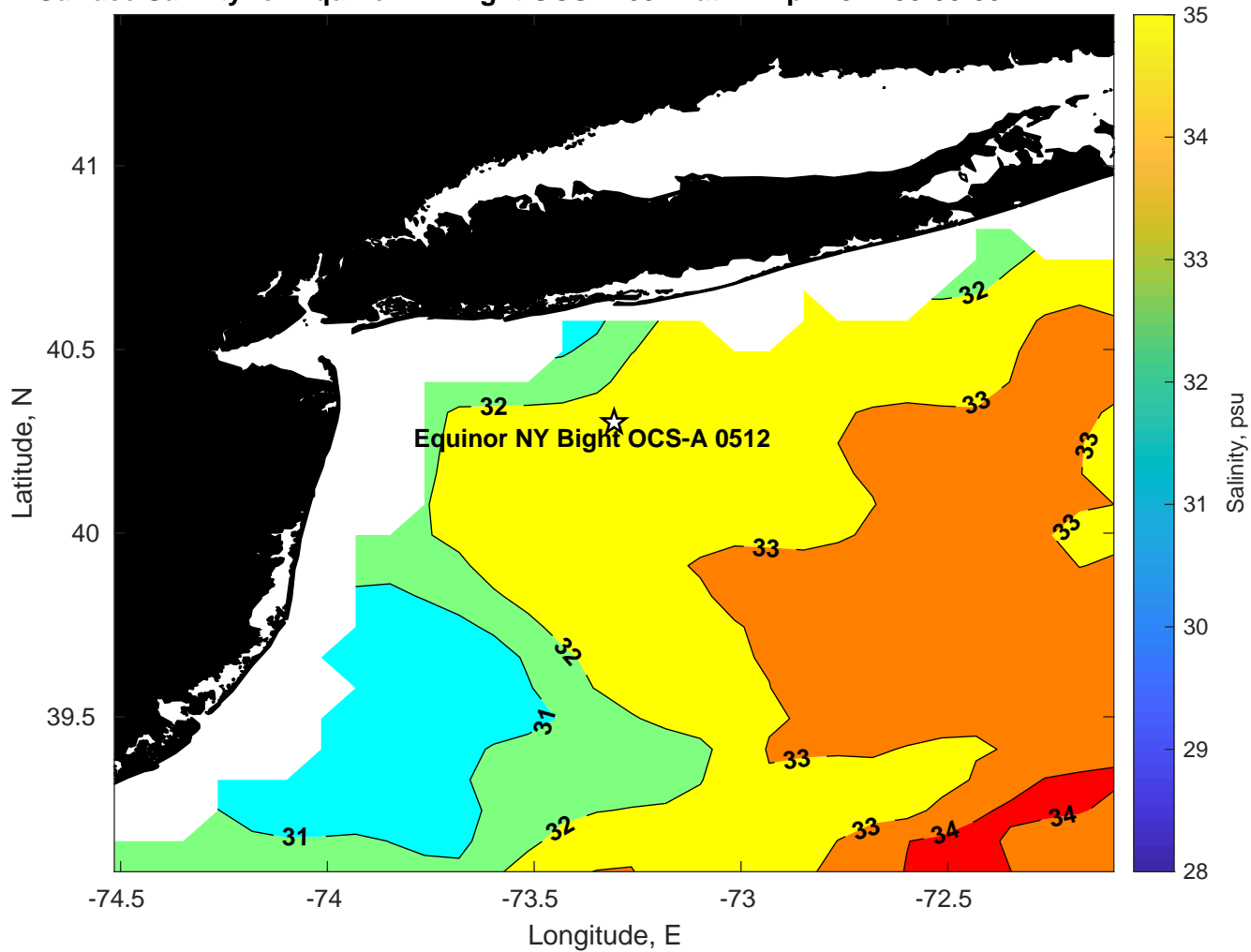
Surface Salinity for Equinor NY Bight OCS-A 0512 at 27-Apr-2024 00:00:00
